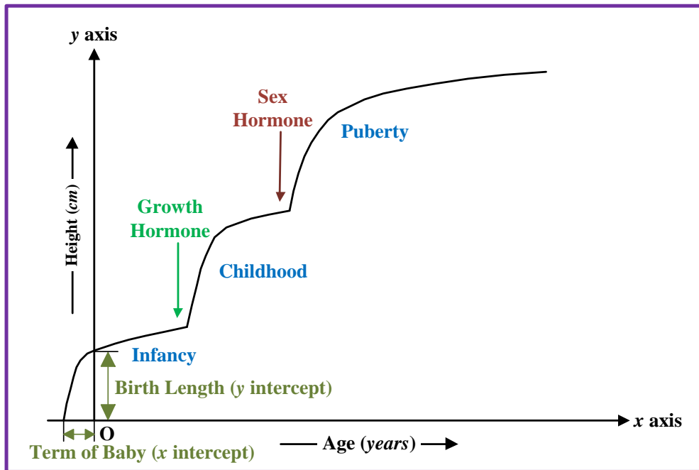
ICP model
